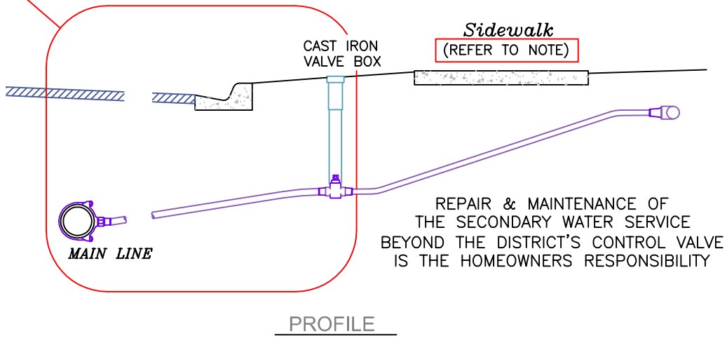
TYPICAL PRE-1990 SECONDARY WATER TURNOUT NOT TO SCALE
